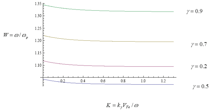
Figure 7: The other dispersion solutions of the equation (18) for different density ratios ( \gamma = 0.2, 0.5, 0.7, 0.9 ).
