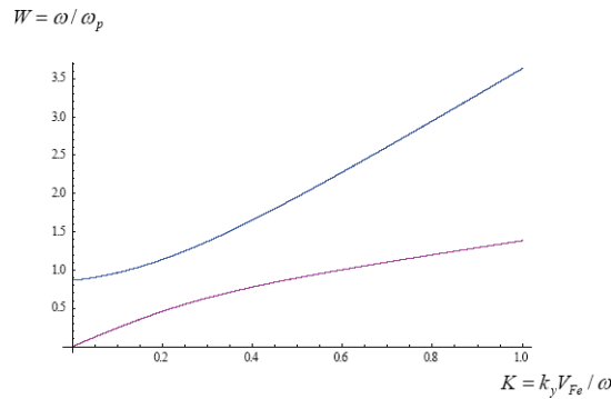
Figure 1: The dispersion relation (5.19) has two positive solutions for positron electron density ratio ( \gamma = 0.5 ) with ( H = 2 ) and ( U = 1 )
