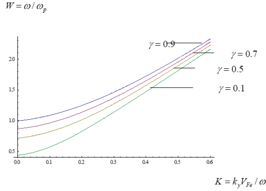
Figure 2: The dispersion relations of the modes for different density positron-electron ratios ( \gamma = 0.1, 0.5, 0.7, 0.9 ) with ( H = 2 ) and ( U = 1 )
