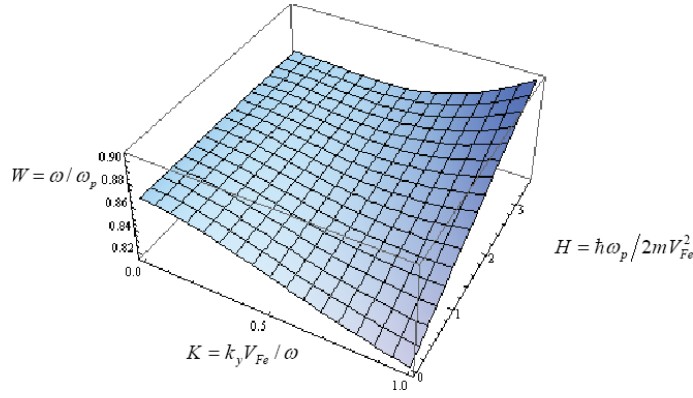
Figure 8: 3D plotting for dispersion relation for perpendicular modes in quantum unmagnetized plasma along quantum ratio axis with ( \gamma = 0.5 , V = 0.2 )
