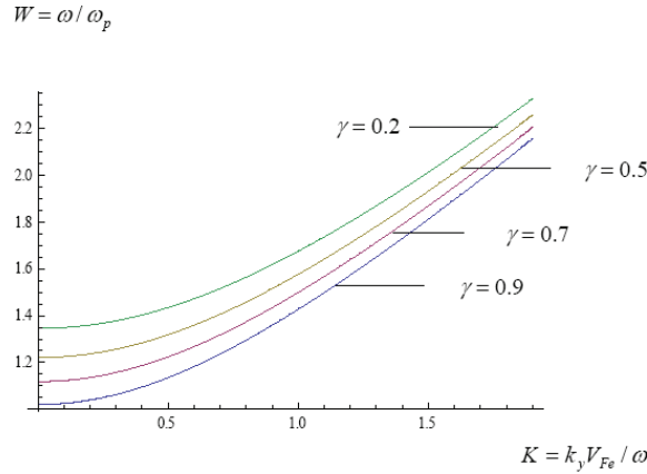
Figure 5: The dispersion relations of electromagnetic modes for different ratios ( \gamma = 0.2, 0.5, 0.7, 0.9 ) in classical plasma.
