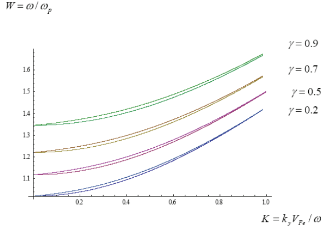
Figure 6: The dispersion solutions of the equations (5.17) and (5.18) for different density ratios ( \gamma = 0.2, 0.5, 0.7, 0.9 ).
