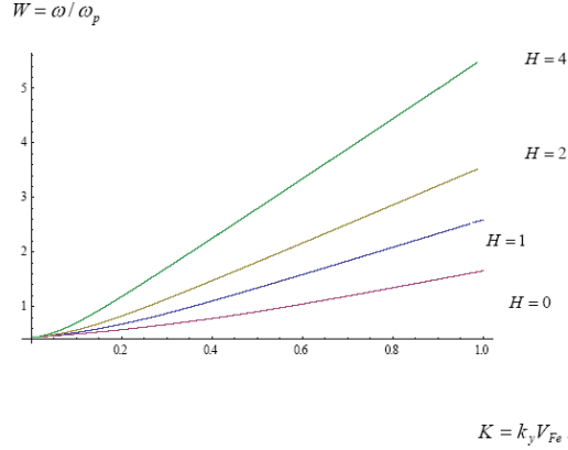
Figure 4: The dispersion relations of different modes for different quantum effects ( H = 0, 1, 2, 4 ) with positron-electron density ratio ( \gamma = 0.9 ) and velocity ratio ( U = 1 ).
