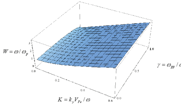
Figure 3: The dispersion relations of the parallel modes along density ratio \gamma -axis with ( H = 2 ) and ( U = 1 )
